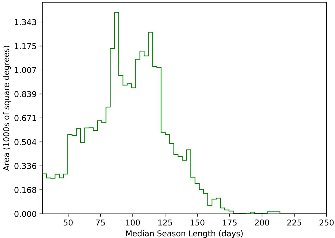
too_elab_r64_d3_gz_v3.4_10yrs All sky g band: Median Season Length
