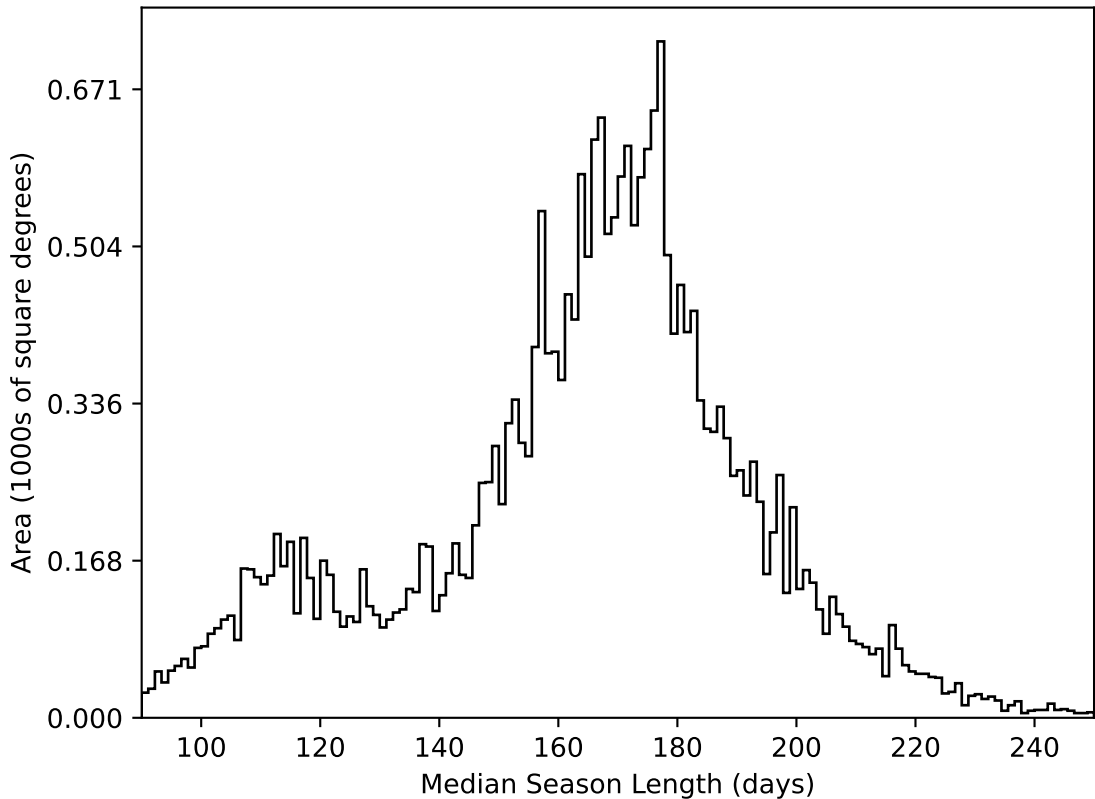
too_elab_r64_d3_gz_v3.4_10yrs All sky all bands: Median Season Length
