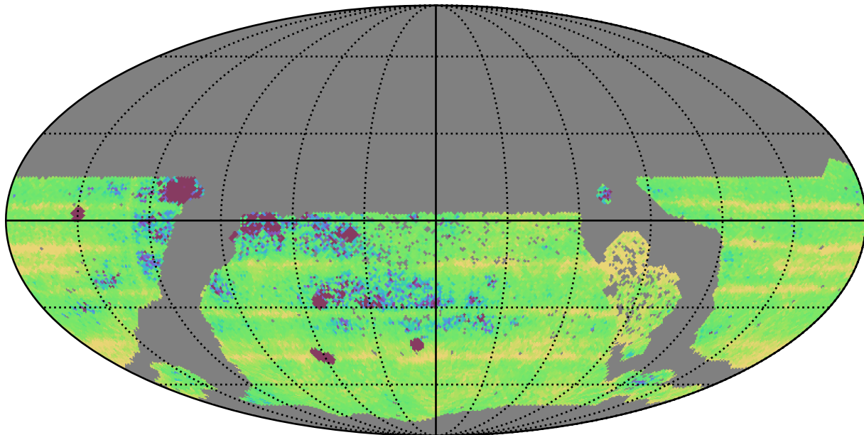
too_elab_r64_d3_gz_v3.4_10yrs WFD: Median Intra-Night Gap
