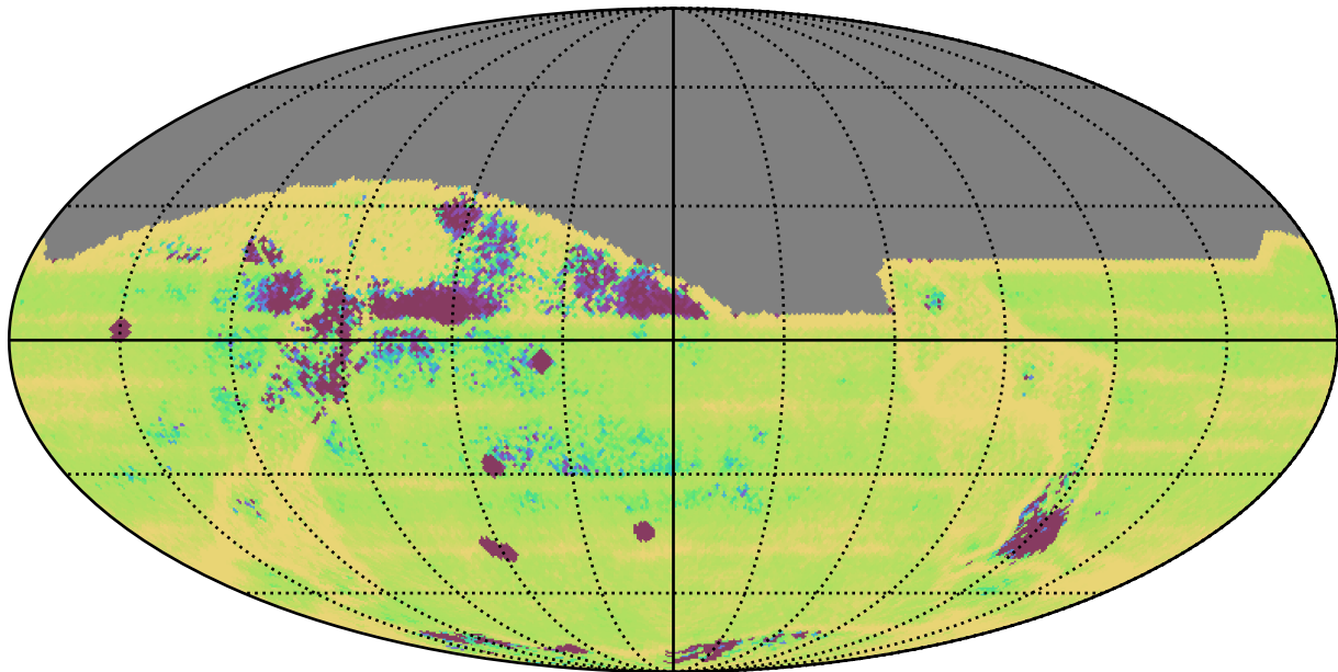
too_elab_r64_d3_gz_v3.4_10yrs All sky: Median Intra-Night Gap
