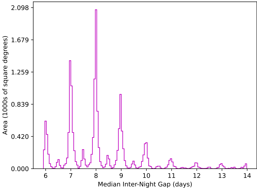
too_elab_r64_d3_gz_v3.4_10yrs WFD z band: Median Inter-Night Gap
