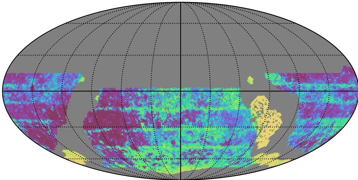
too_elab_r64_d3_gz_v3.4_10yrs WFD y band: Median Inter-Night Gap
