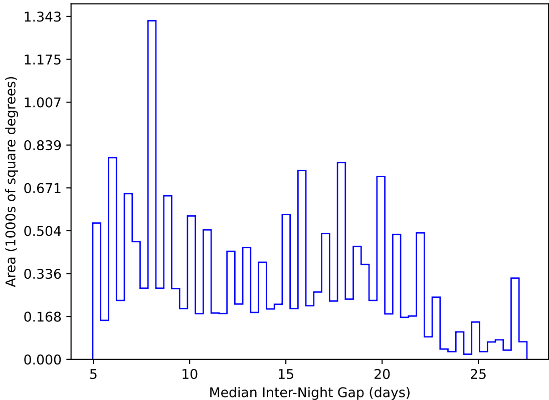
too_elab_r64_d3_gz_v3.4_10yrs WFD y band: Median Inter-Night Gap
