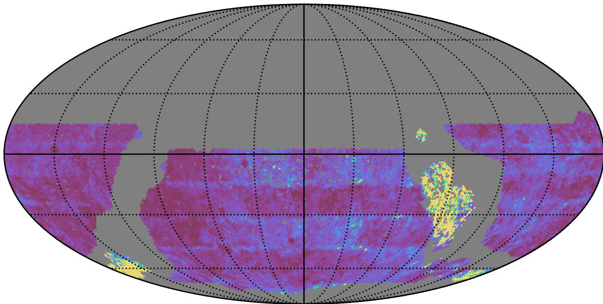
too_elab_r64_d3_gz_v3.4_10yrs WFD u band: Median Inter-Night Gap
