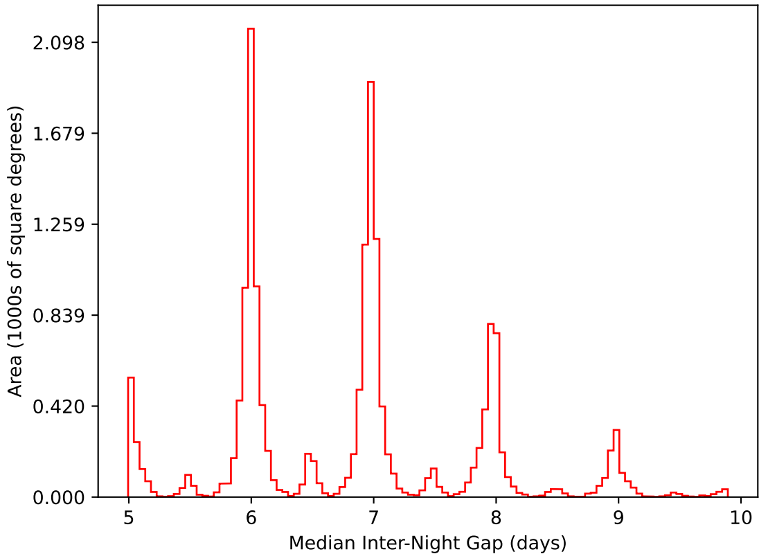
too_elab_r64_d3_gz_v3.4_10yrs WFD i band: Median Inter-Night Gap
