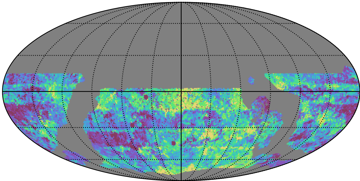
too_elab_r64_d3_gz_v3.4_10yrs WFD g band: Median Inter-Night Gap
