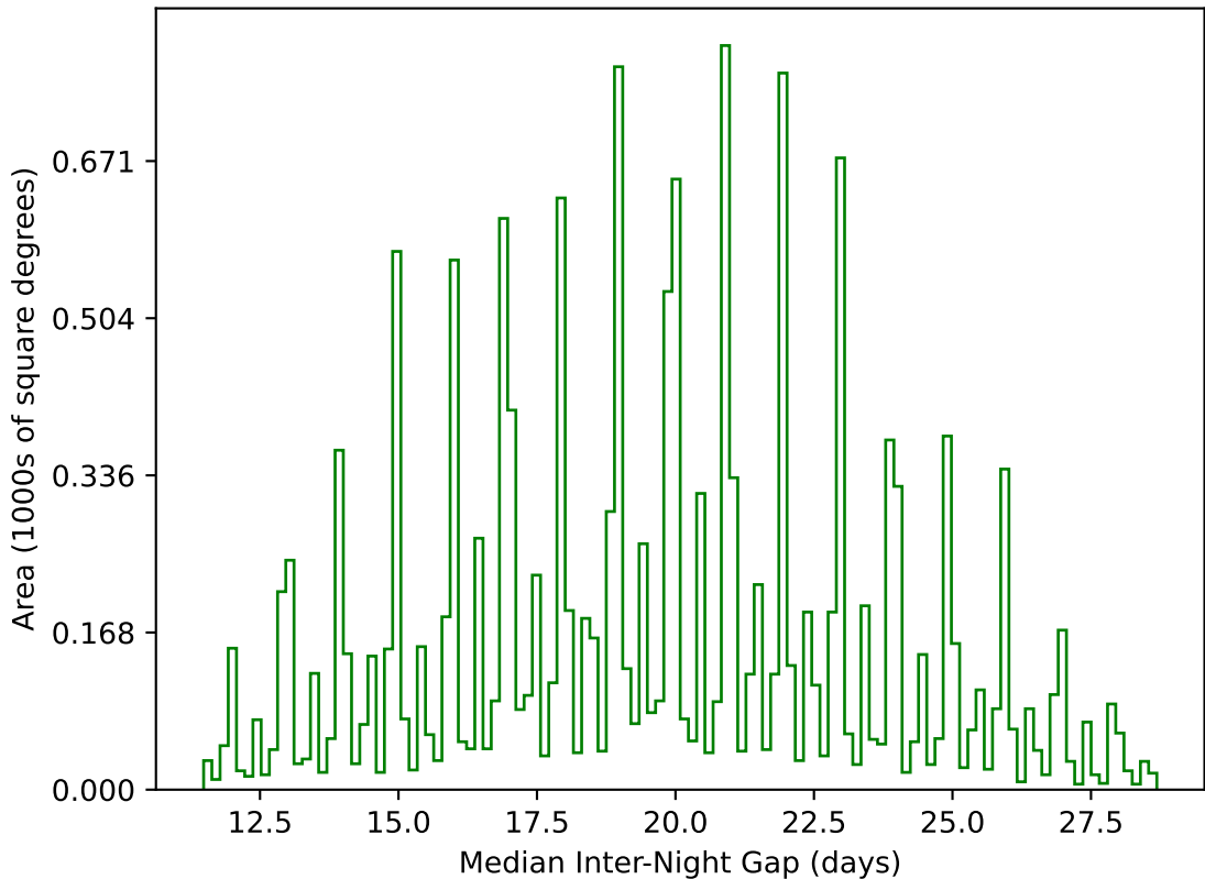
too_elab_r64_d3_gz_v3.4_10yrs WFD g band: Median Inter-Night Gap
