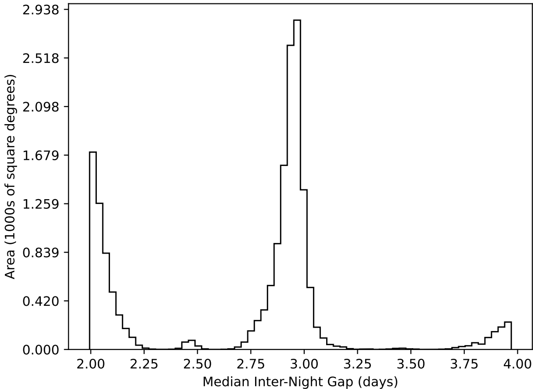
too_elab_r64_d3_gz_v3.4_10yrs WFD all bands: Median Inter-Night Gap
