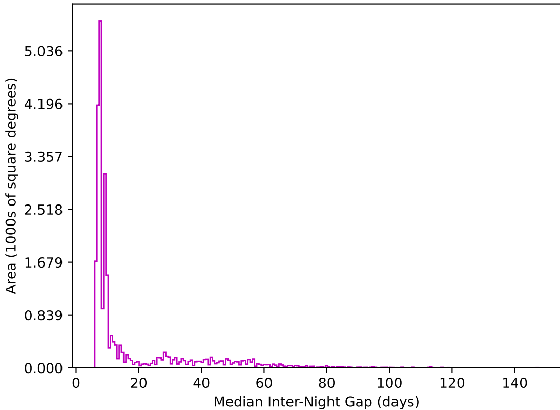
too_elab_r64_d3_gz_v3.4_10yrs All sky z band: Median Inter-Night Gap
