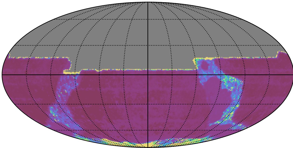
too_elab_r64_d3_gz_v3.4_10yrs All sky y band: Median Inter-Night Gap
