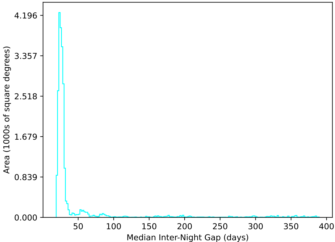
too_elab_r64_d3_gz_v3.4_10yrs All sky u band: Median Inter-Night Gap
