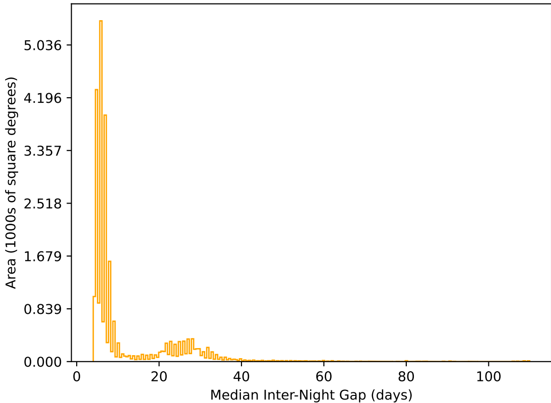
too_elab_r64_d3_gz_v3.4_10yrs All sky r band: Median Inter-Night Gap
