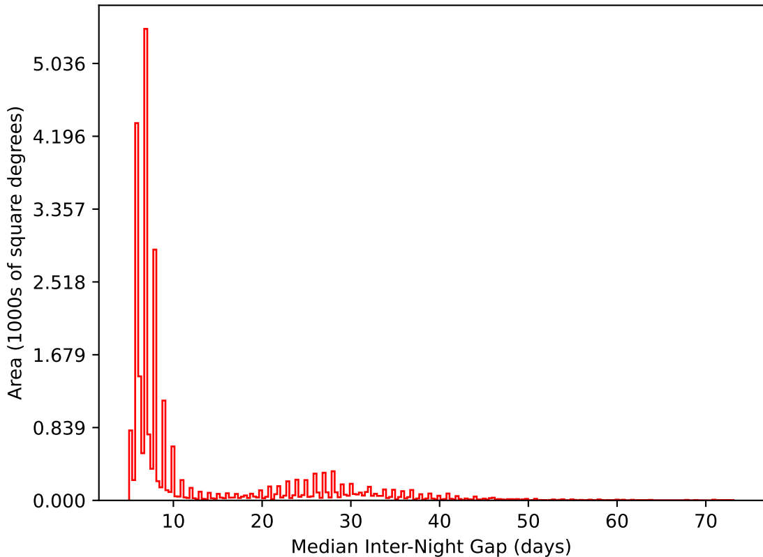
too_elab_r64_d3_gz_v3.4_10yrs All sky i band: Median Inter-Night Gap
