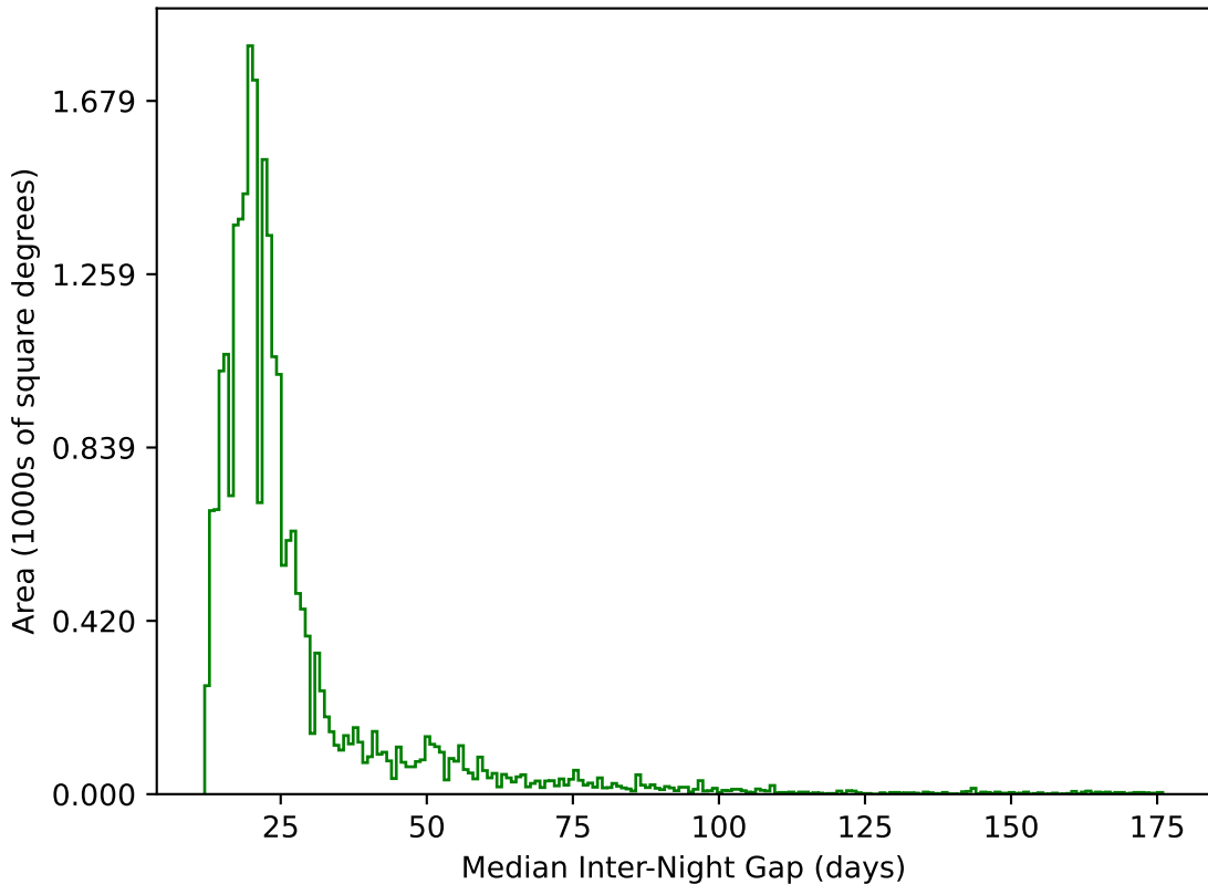
too_elab_r64_d3_gz_v3.4_10yrs All sky g band: Median Inter-Night Gap
