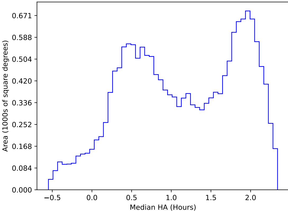
too_elab_r64_d3_gz_v3.4_10yrs WFD z band: Median HA
