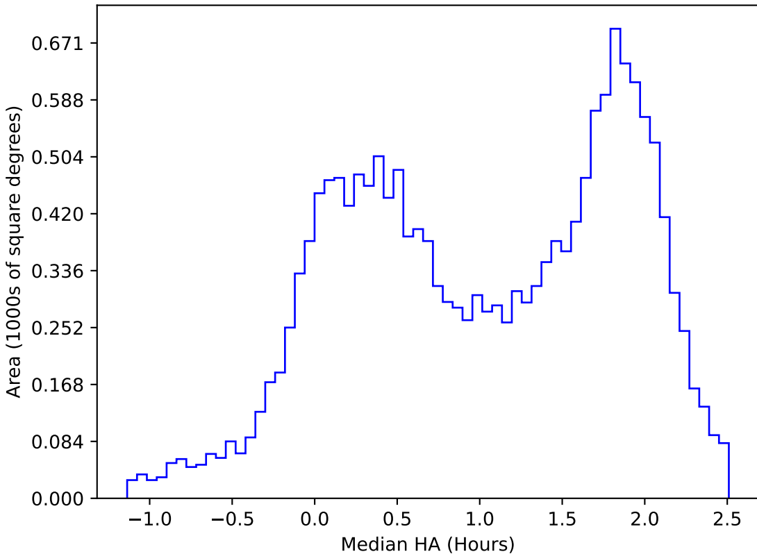
too_elab_r64_d3_gz_v3.4_10yrs WFD u band: Median HA
