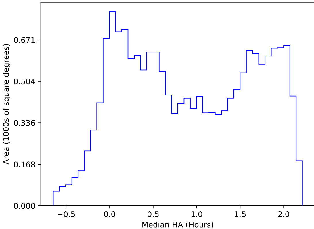
too_elab_r64_d3_gz_v3.4_10yrs WFD r band: Median HA
