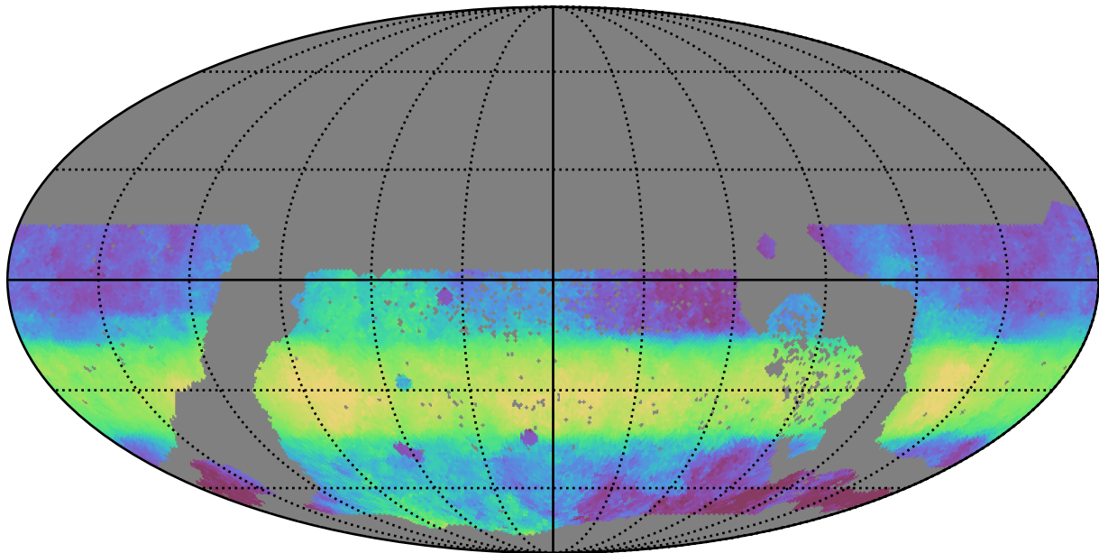
too_elab_r64_d3_gz_v3.4_10yrs WFD i band: Median HA
