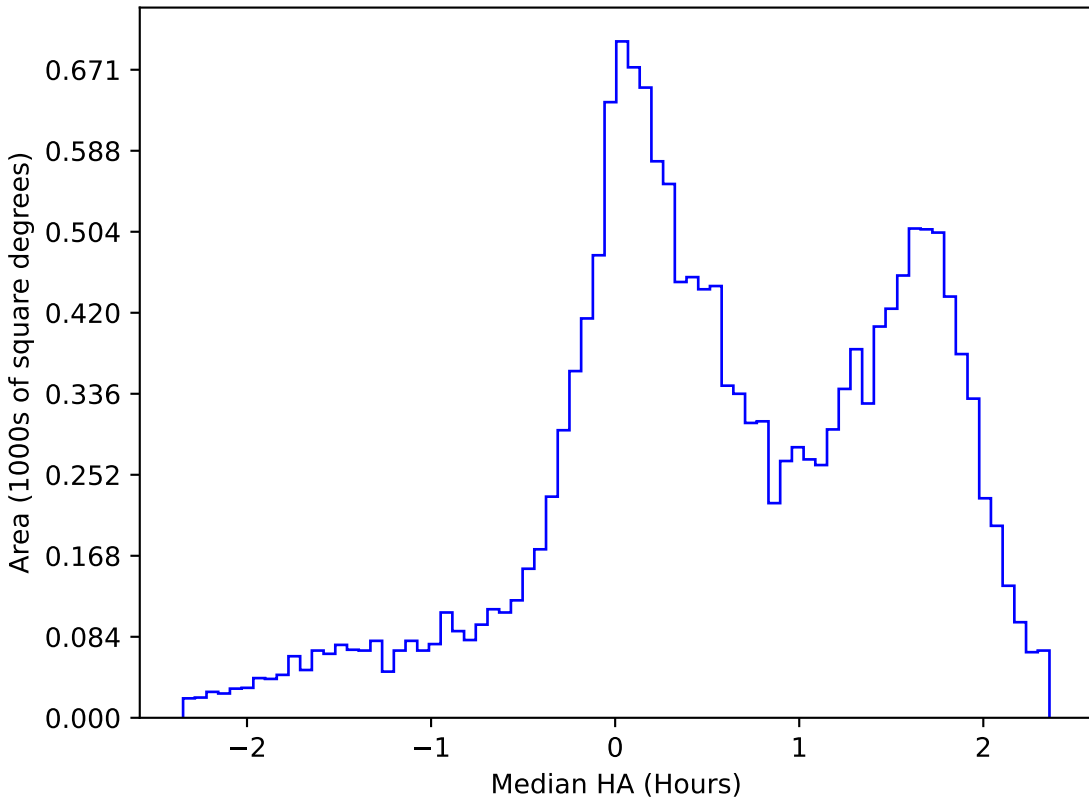
too_elab_r64_d3_gz_v3.4_10yrs WFD g band: Median HA
