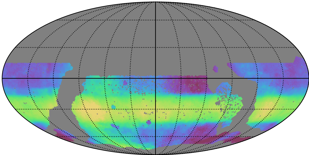
too_elab_r64_d3_gz_v3.4_10yrs WFD all bands: Median HA
