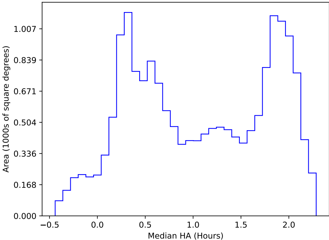
too_elab_r64_d3_gz_v3.4_10yrs WFD all bands: Median HA
