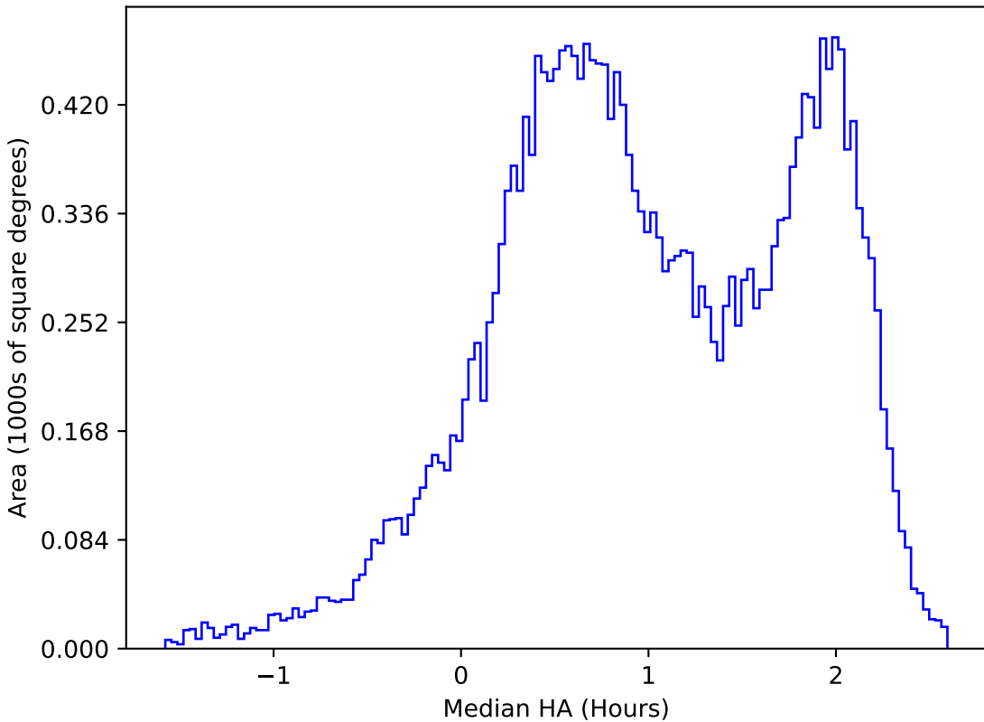
too_elab_r64_d3_gz_v3.4_10yrs All sky z band: Median HA
