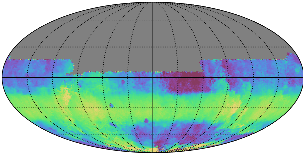
too_elab_r64_d3_gz_v3.4_10yrs All sky y band: Median HA
