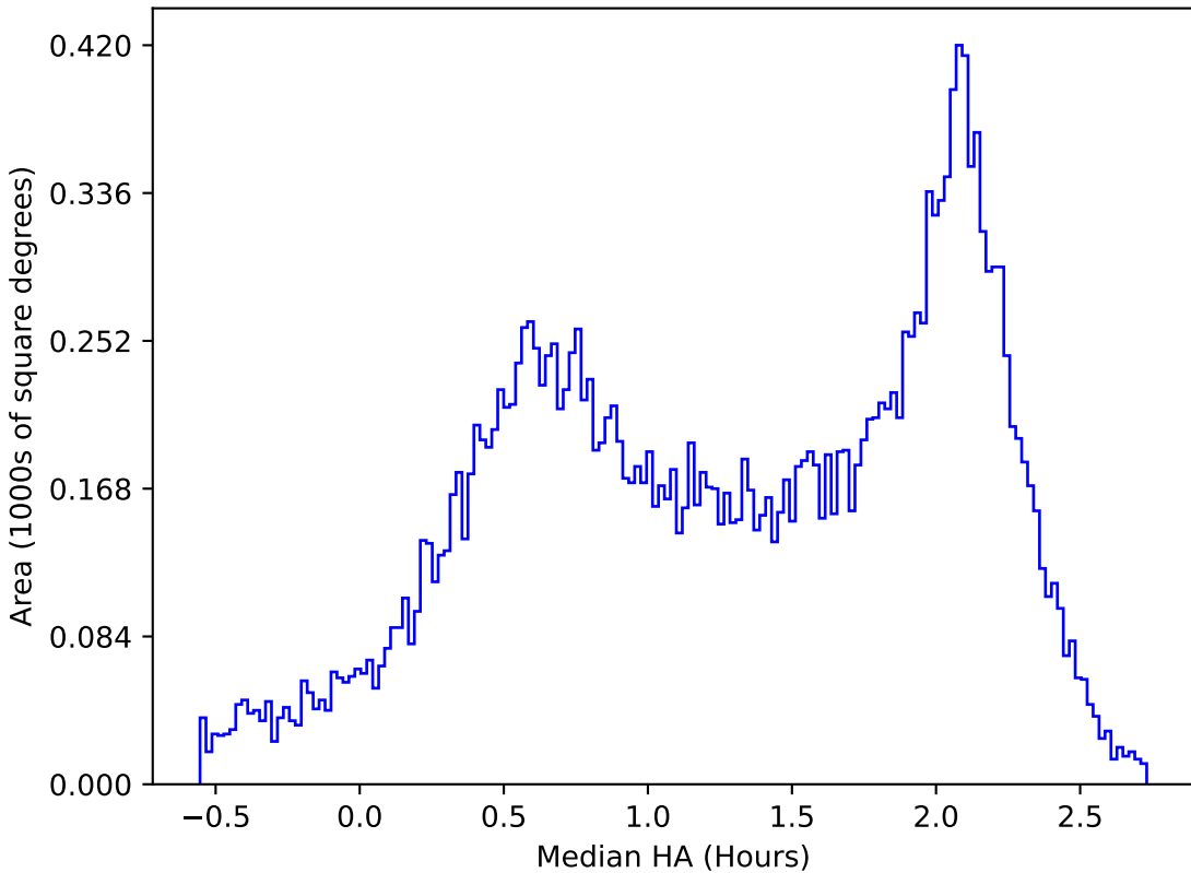
too_elab_r64_d3_gz_v3.4_10yrs All sky y band: Median HA
