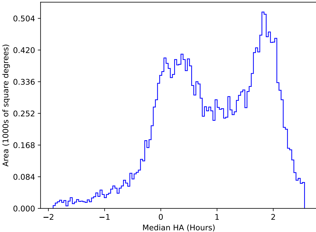
too_elab_r64_d3_gz_v3.4_10yrs All sky u band: Median HA
