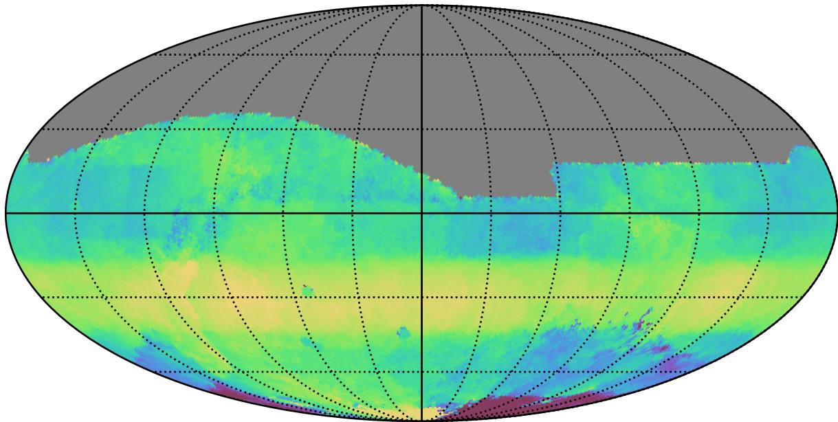
too_elab_r64_d3_gz_v3.4_10yrs All sky r band: Median HA
