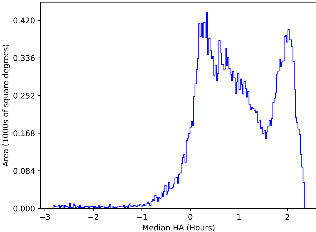
too_elab_r64_d3_gz_v3.4_10yrs All sky i band: Median HA
