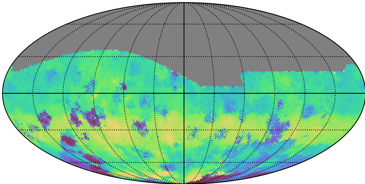
too_elab_r64_d3_gz_v3.4_10yrs All sky g band: Median HA
