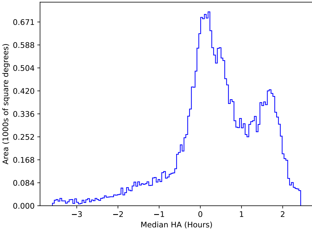
too_elab_r64_d3_gz_v3.4_10yrs All sky g band: Median HA
