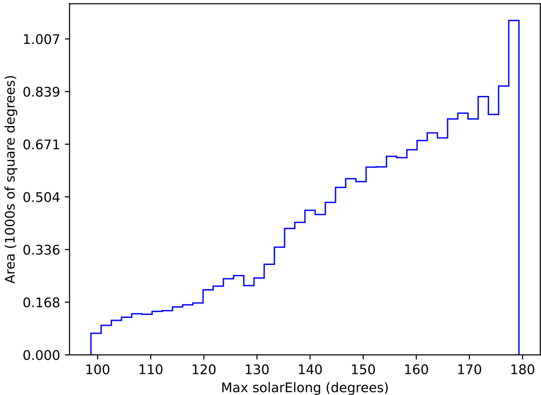
too_elab_r64_d3_gz_v3.4_10yrs WFD z band: Max solarElong
