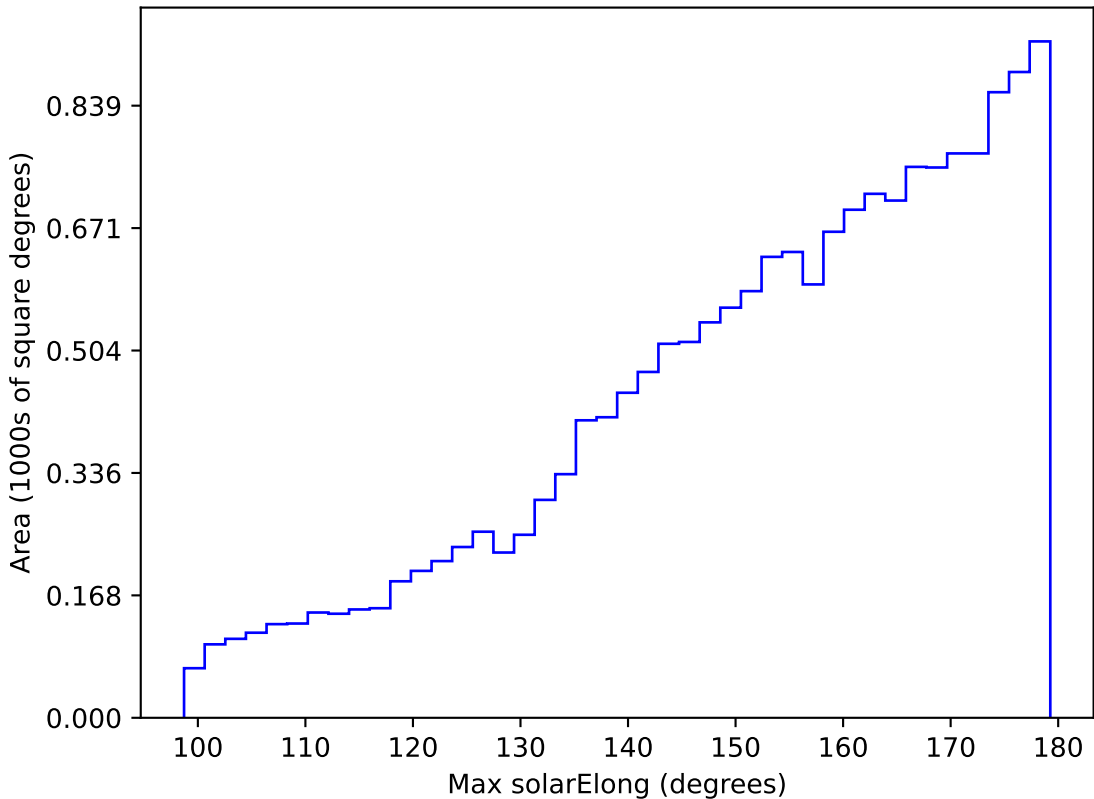
too_elab_r64_d3_gz_v3.4_10yrs WFD y band: Max solarElong
