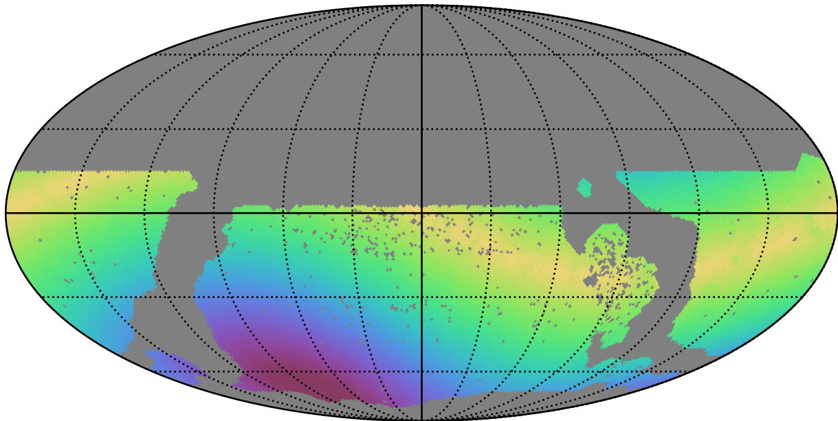
too_elab_r64_d3_gz_v3.4_10yrs WFD u band: Max solarElong
