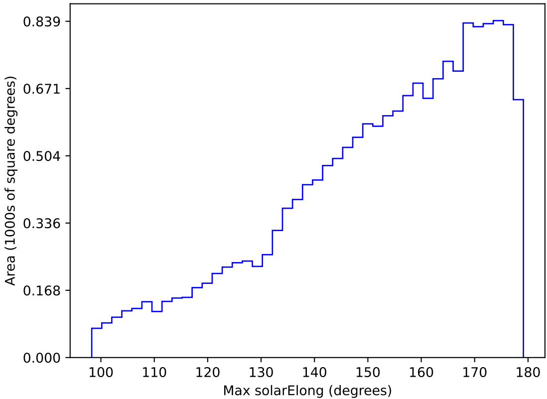
too_elab_r64_d3_gz_v3.4_10yrs WFD u band: Max solarElong
