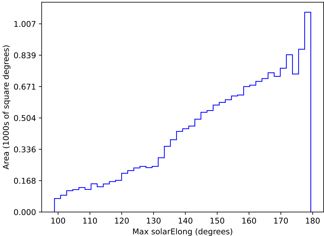
too_elab_r64_d3_gz_v3.4_10yrs WFD i band: Max solarElong
