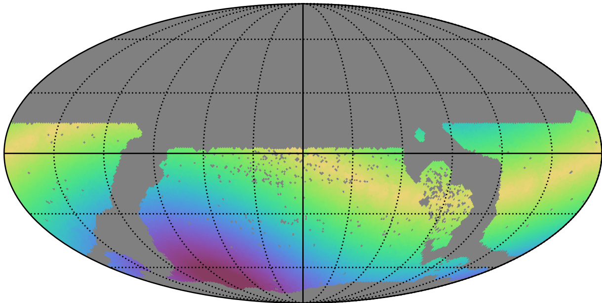
too_elab_r64_d3_gz_v3.4_10yrs WFD g band: Max solarElong
