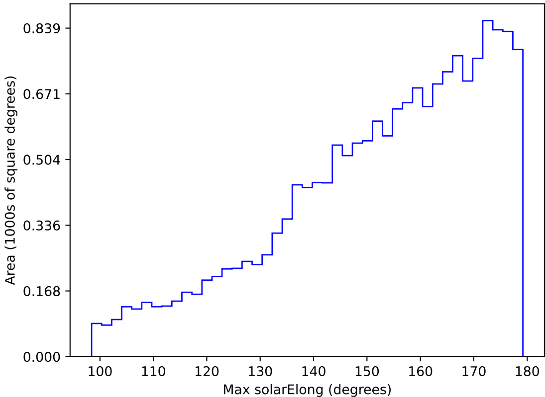
too_elab_r64_d3_gz_v3.4_10yrs WFD g band: Max solarElong
