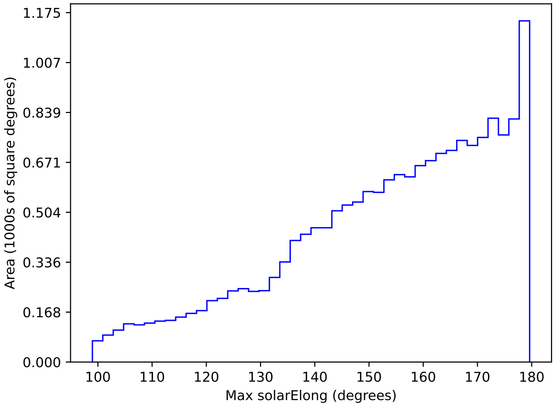
too_elab_r64_d3_gz_v3.4_10yrs WFD all bands: Max solarElong
