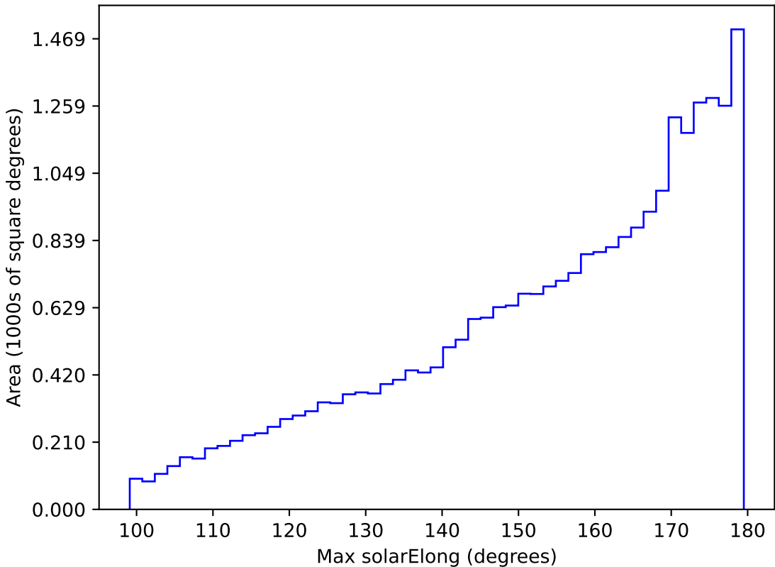
too_elab_r64_d3_gz_v3.4_10yrs All sky r band: Max solarElong
