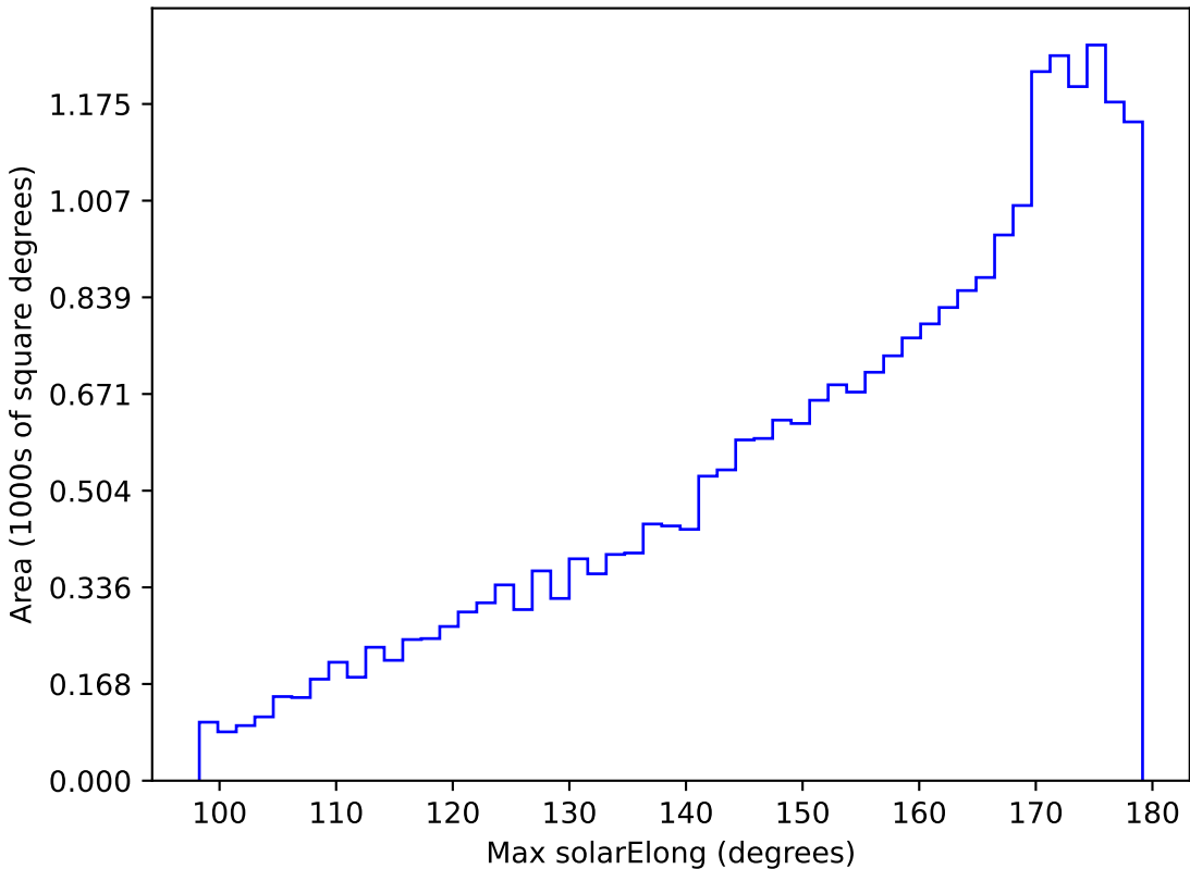
too_elab_r64_d3_gz_v3.4_10yrs All sky g band: Max solarElong
