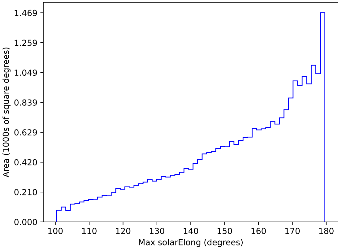
too_elab_r64_d3_gz_v3.4_10yrs All sky all bands: Max solarElong
