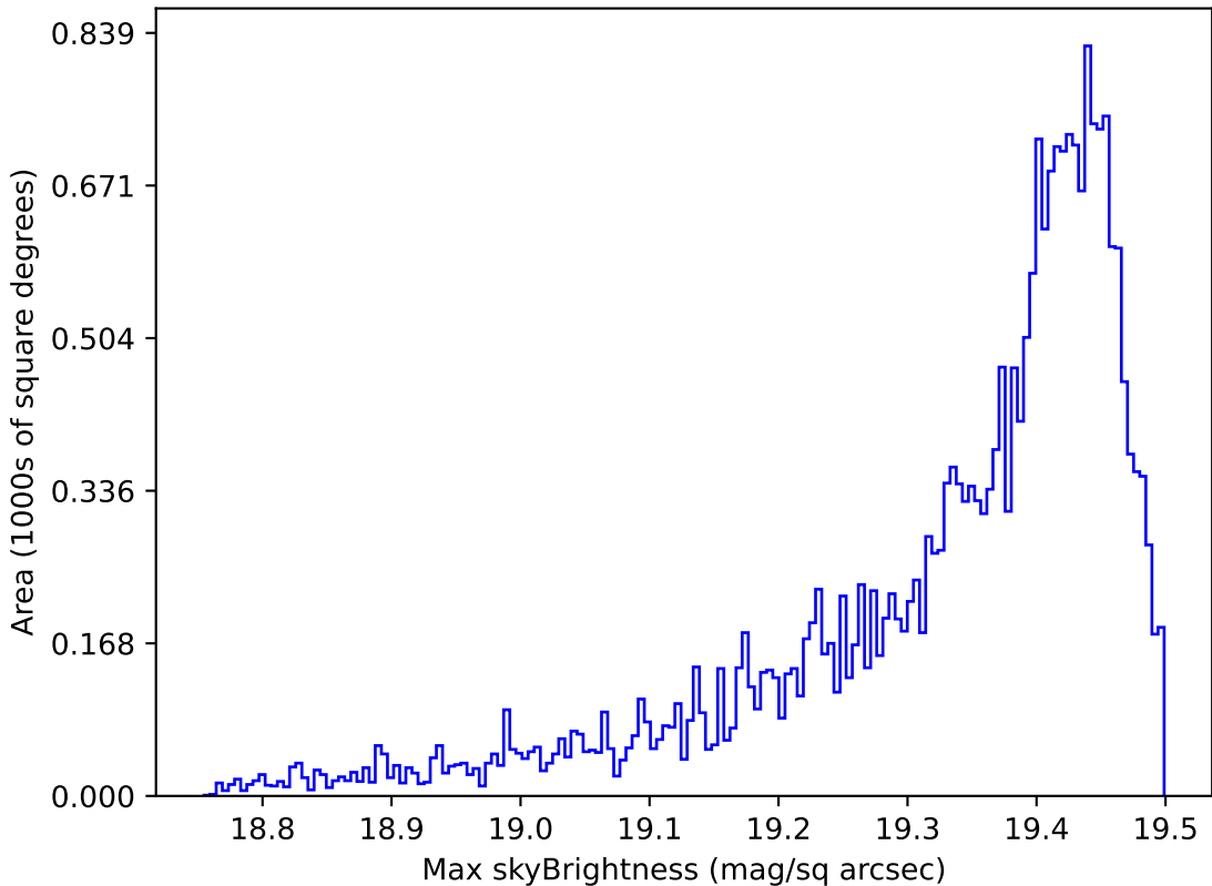
too_elab_r64_d3_gz_v3.4_10yrs Yr 1 z band: Max skyBrightness
