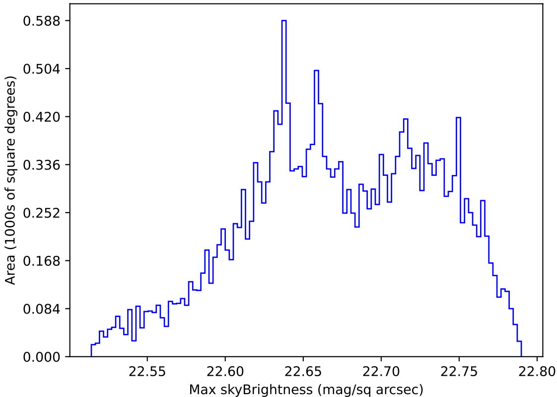
too_elab_r64_d3_gz_v3.4_10yrs Yr 1 u band: Max skyBrightness
