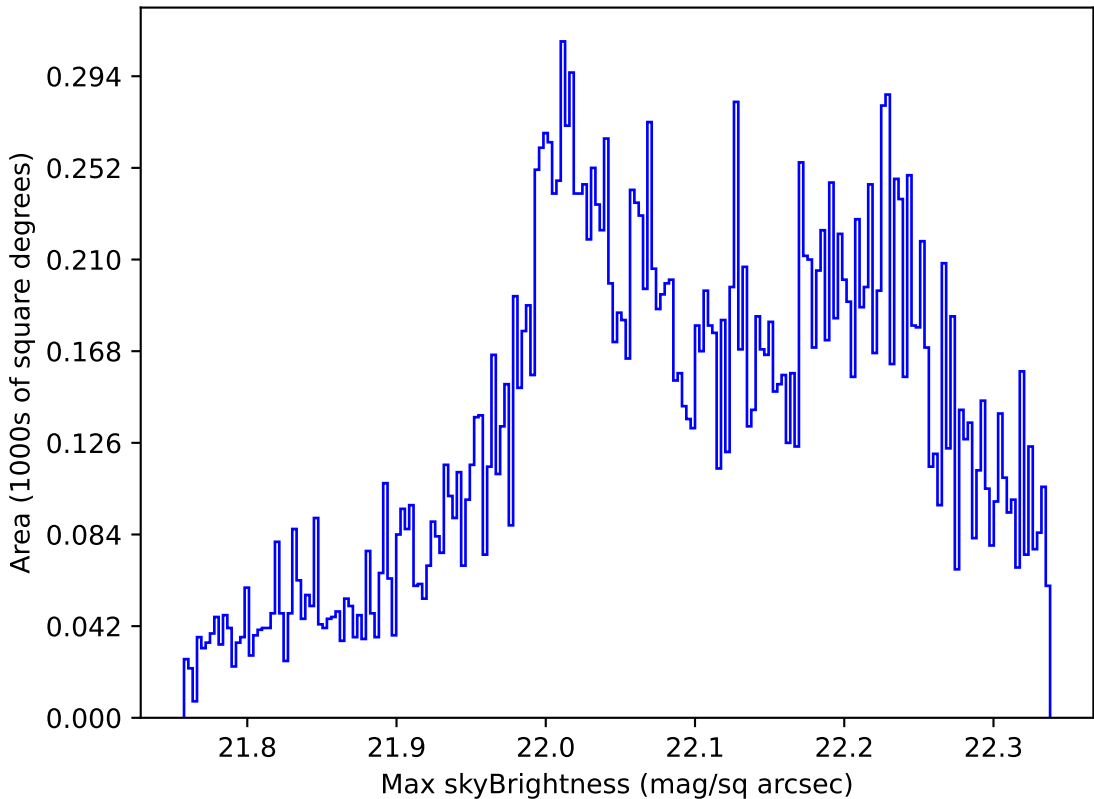
too_elab_r64_d3_gz_v3.4_10yrs Yr 1 g band: Max skyBrightness
