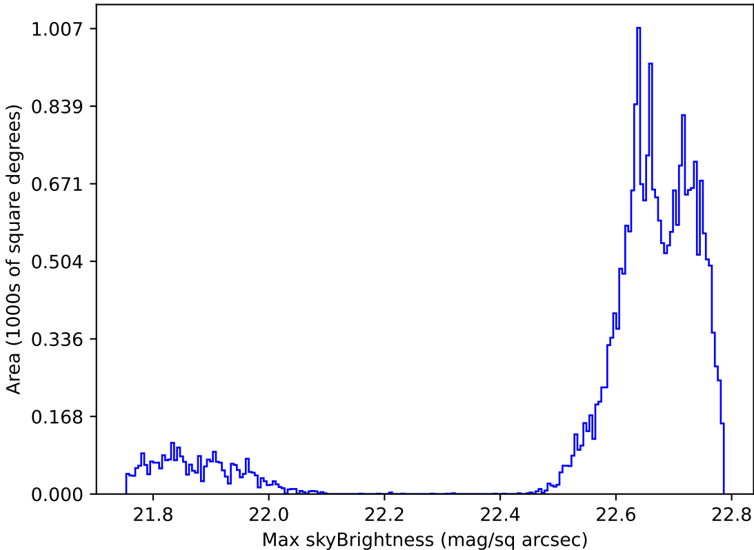
too_elab_r64_d3_gz_v3.4_10yrs Yr 1 all bands: Max skyBrightness
