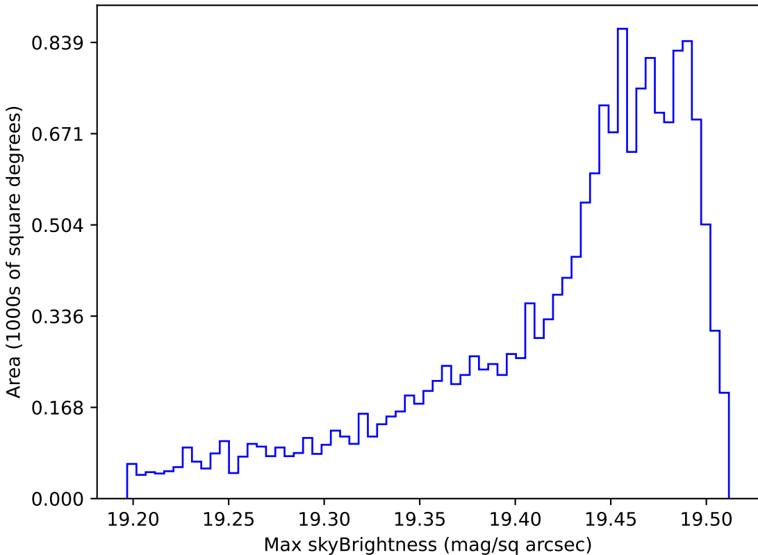
too_elab_r64_d3_gz_v3.4_10yrs WFD z band: Max skyBrightness
