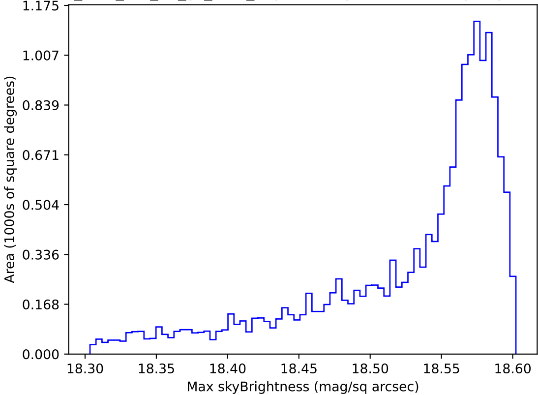
too_elab_r64_d3_gz_v3.4_10yrs WFD y band: Max skyBrightness
